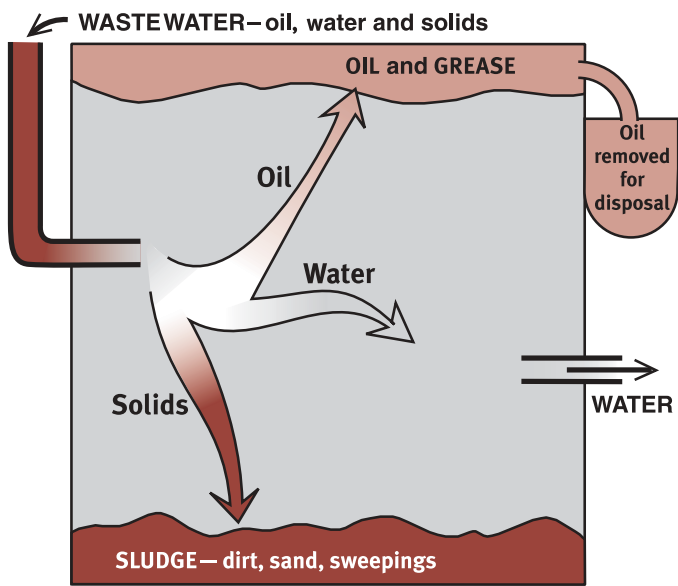
Simplified diagram of OWS operation
